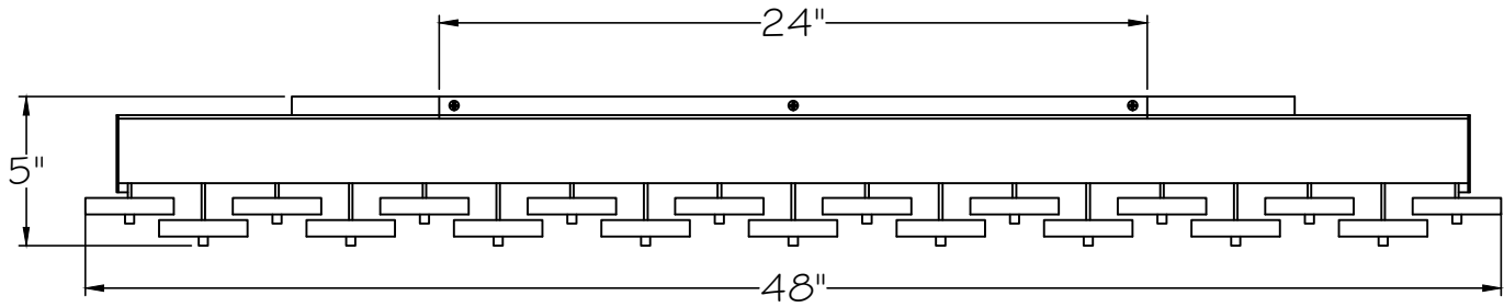
TOP VIEW
